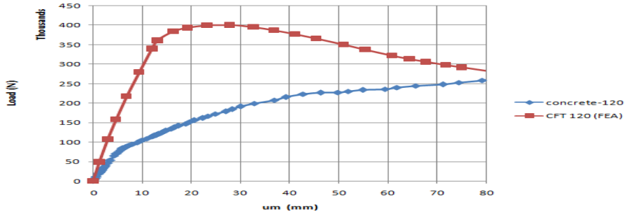
Fig-12. Load-mid span lateral deflection curve of reinforced concrete
