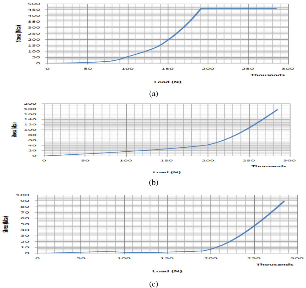
Fig-13. Load-stress curve for (a) steel rebar in tension (b) concrete in compression (c) concrete in tension
