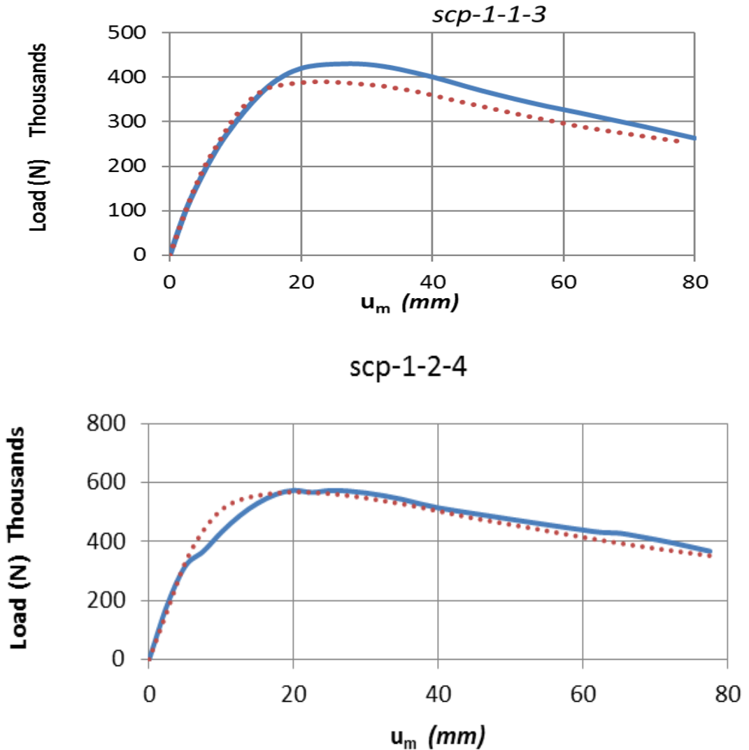
Fig-2. Load versus mid-span lateral deflection curves (Experimental curves are shown in solid lines; Predicted curves are shown in dashed lines)
