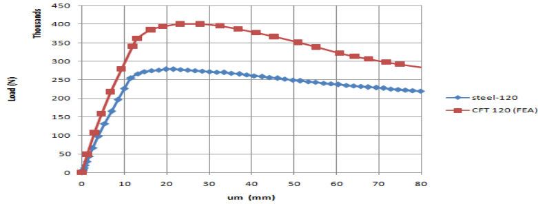
Fig-14. Load-Mid Span Lateral Deflection Curve of Steel Tube
